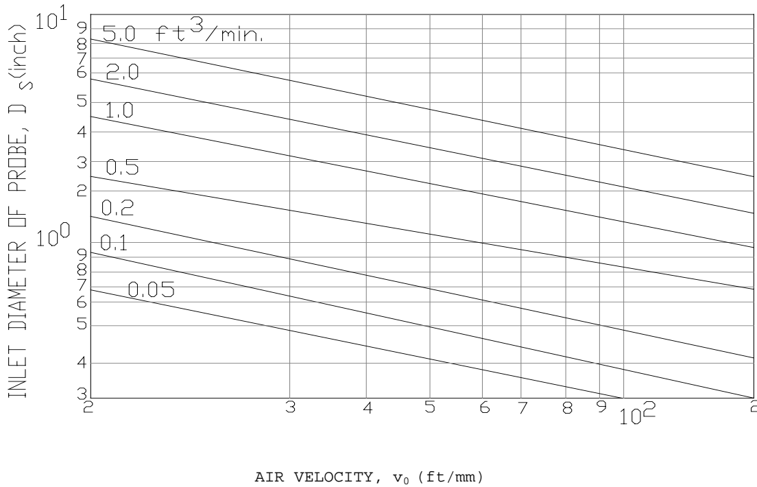
Figure C.2. Probe inlet diameters (English units) for isokinetic sampling, \mathbf{v} = \mathbf{v}_0 (volumetric flow rates shown parametrically)
