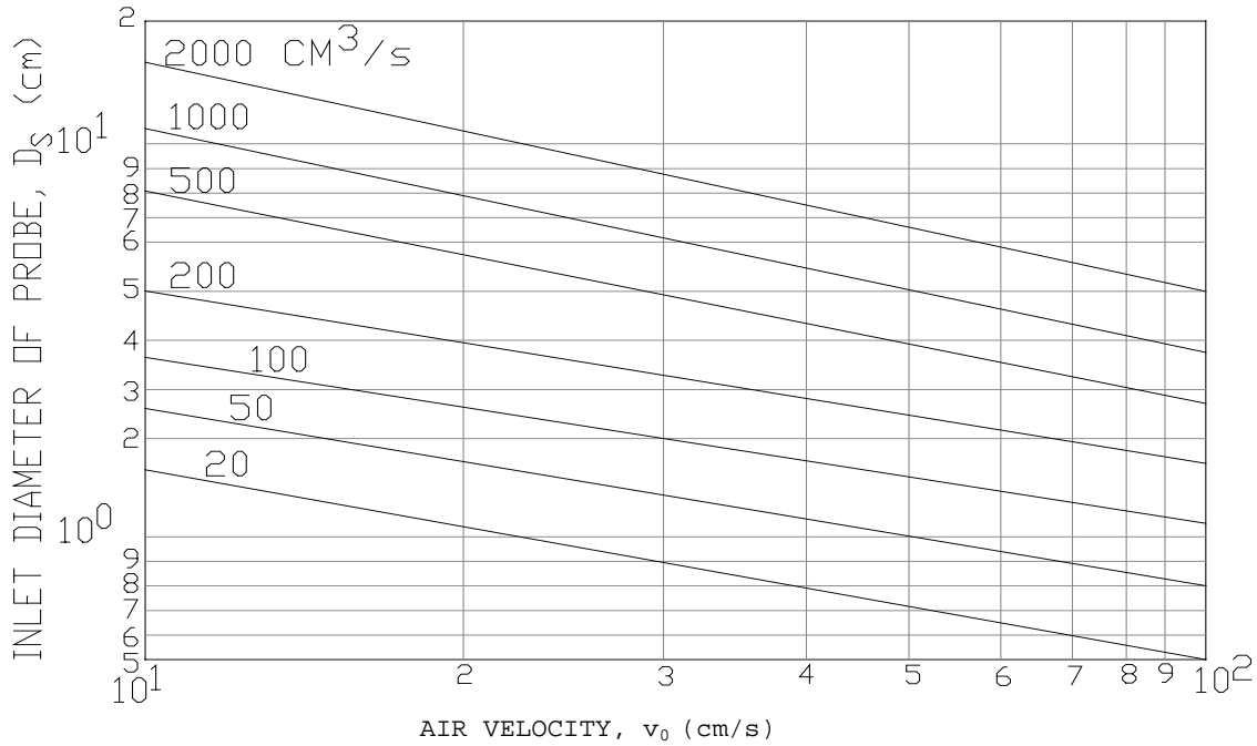
Figure C.1. Probe inlet diameters (metric units) for isokinetic sampling, \mathbf{v} = \mathbf{v}_0 (volumetric flow rates shown parametrically)
